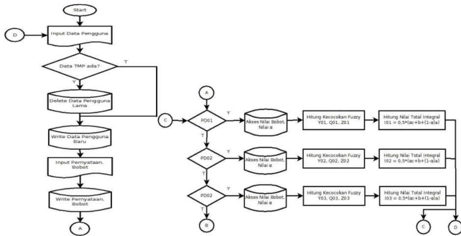
Gambar 6. Flowchart sistem.
