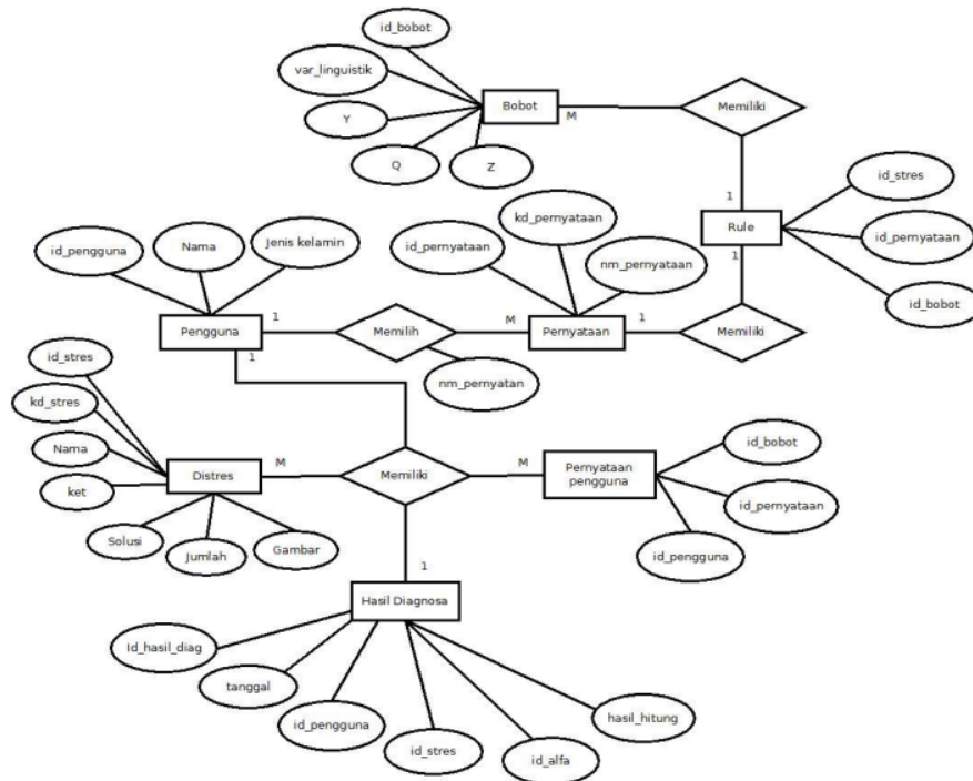
Gambar 7. Entity relationship diagram (ERD).
